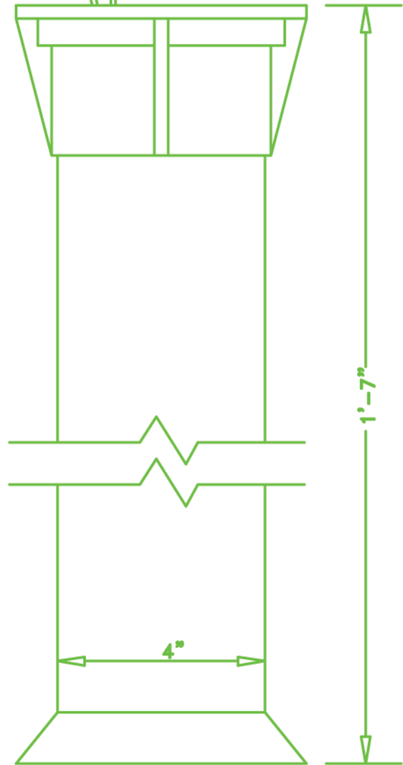
SIDE VIEW OF BARREL
