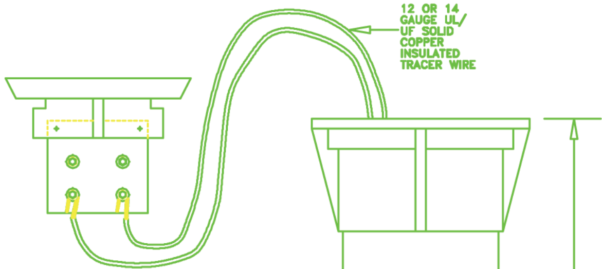
SIDE VIEW OF CAP
